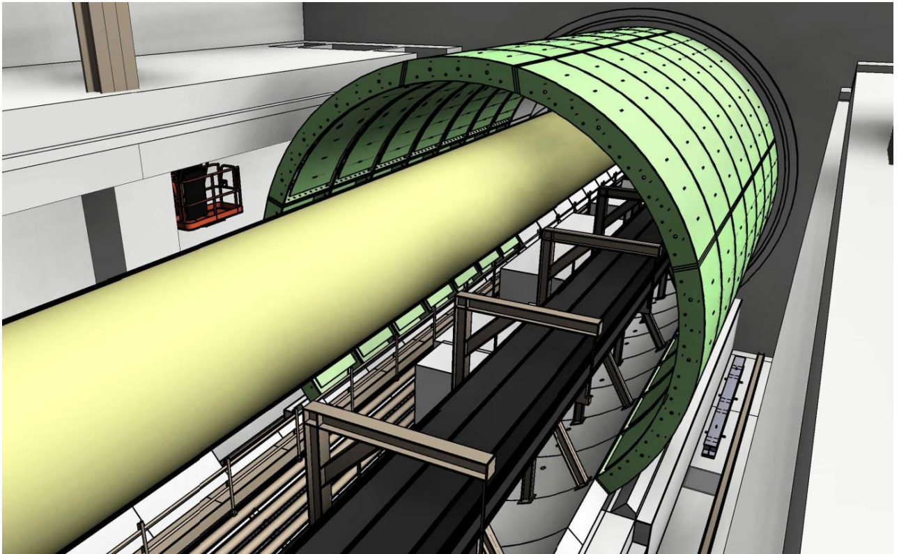
3D visualisation of the tunnel model for Lot 3 of Line C of the Toulouse Metro (image: ©Implenia).
